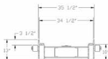
HOIST FRAME DETAIL
